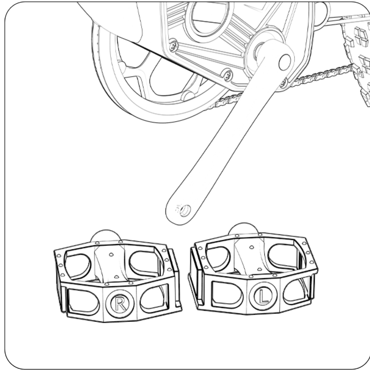
12. When installing the foot pedal, pay attention to distinguishing between "R" and "L".
